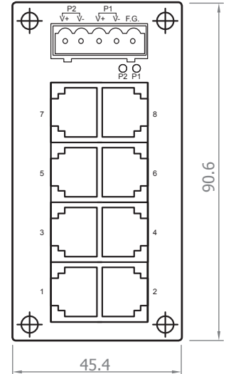
Front-panel view
