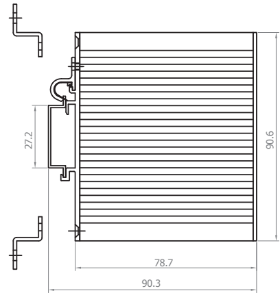
Housing side view
